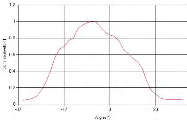
RADIATION DISTRIBUTION
